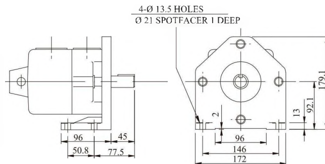
Foot Type (脚座型)
