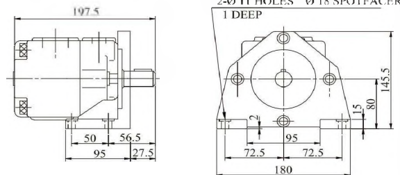
Foot Type (脚座型)
