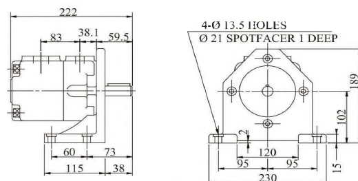
Foot Type (脚座型)
