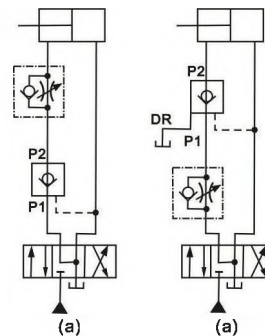
Internal drain
