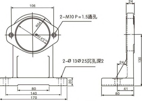
SGP1A腳座 SGP1A Foot
