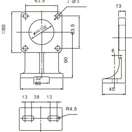
SGP1A腳座 SGP1A Foot
